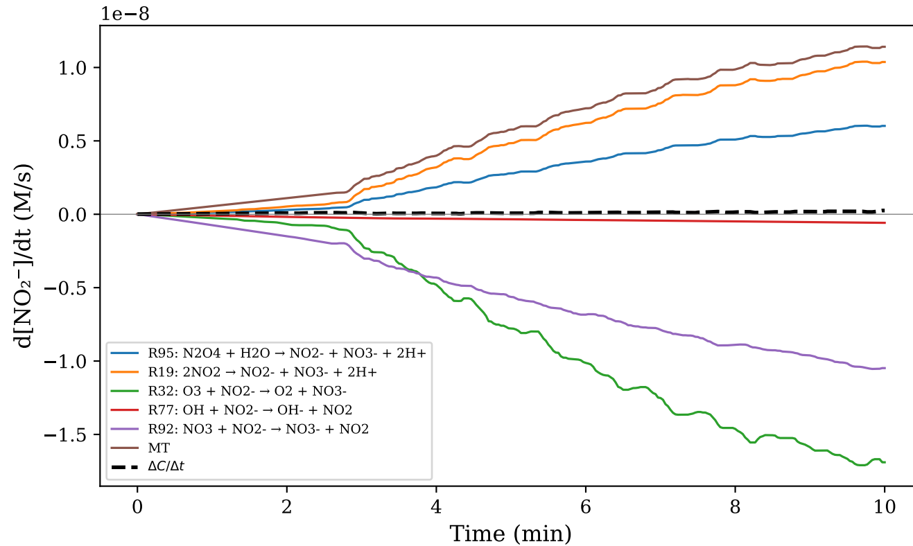
(c) \text{NO}_2^-
