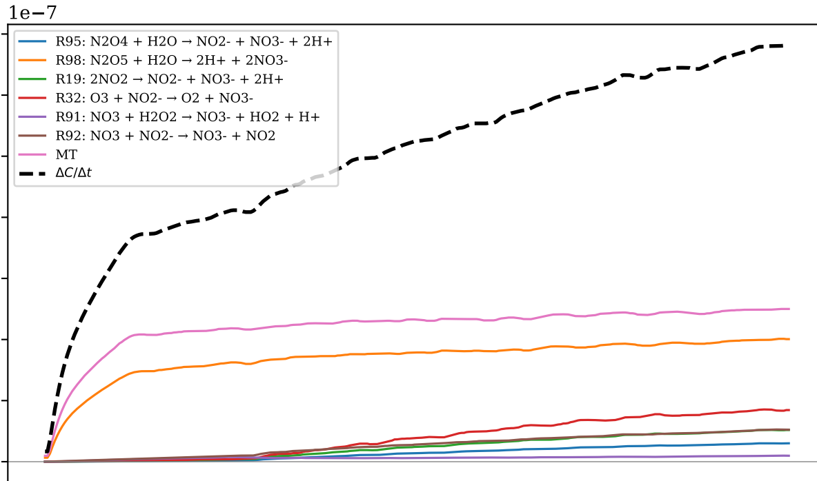
(a) \text{NO}_3^-
